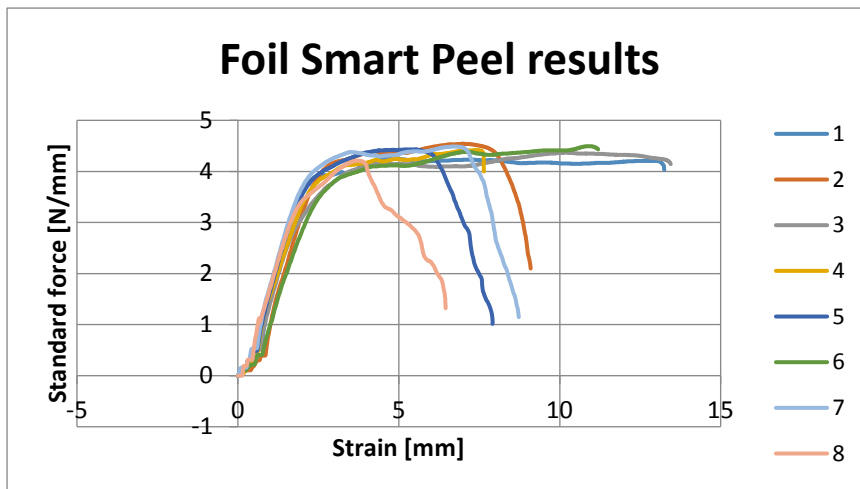
Figure 1: results from the eight peel adhesions
